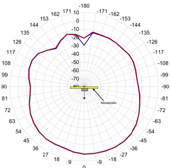
LTE 2600 MHz
