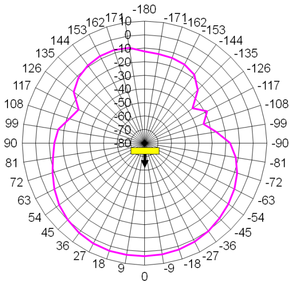
LTE 2600 MHz
